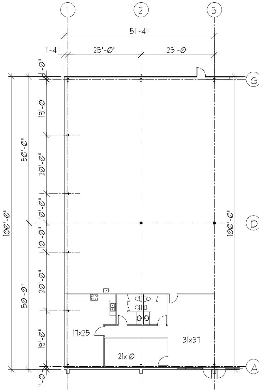
FLOOR PLAN BAYS 1-3
