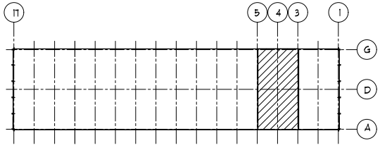
LOCATION PLAN BAYS 3-5
