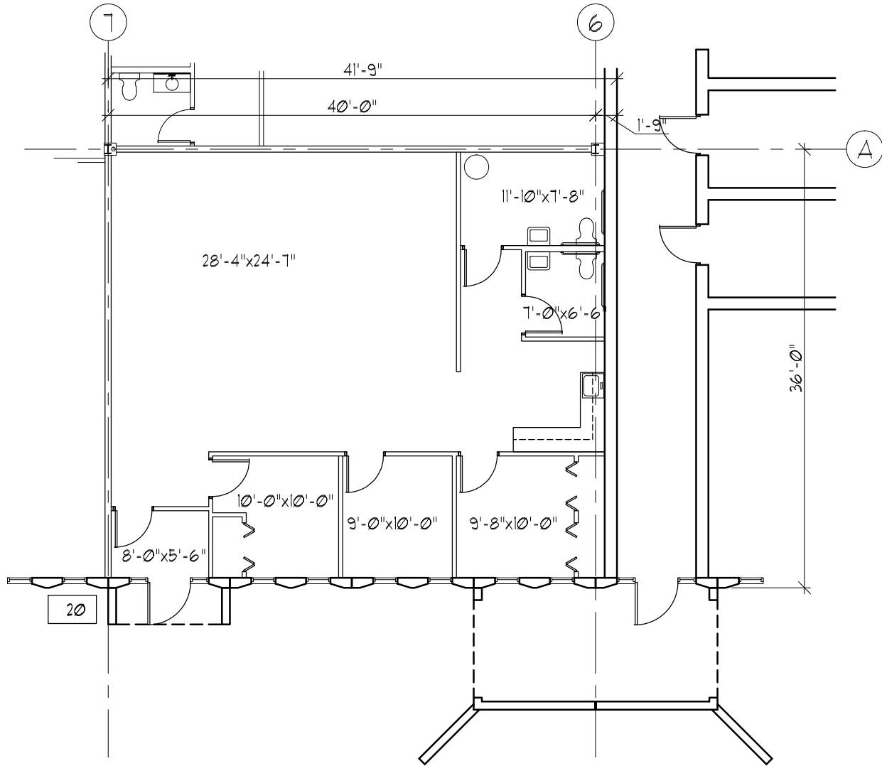
FLOOR PLAN 1,503 SF
