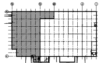
LOCATION PLAN BAYS 10-19
